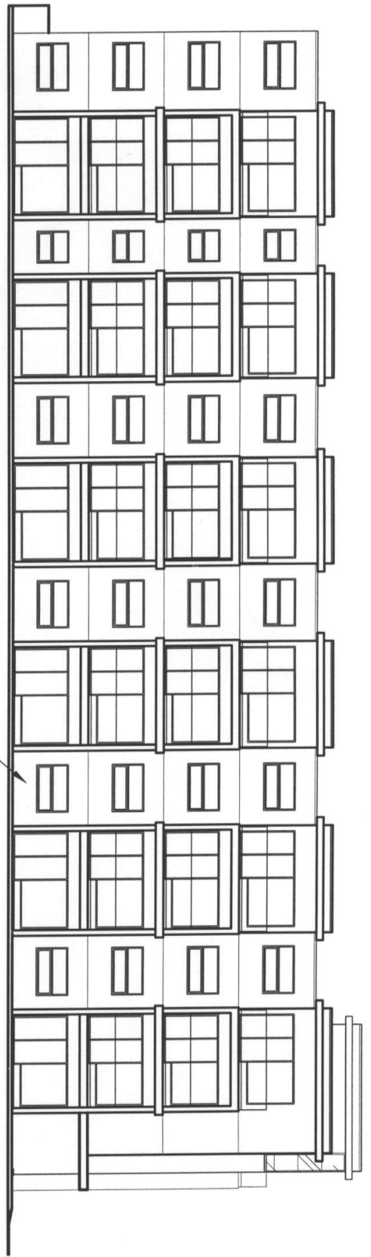
EAST (112 Street) ELEVATION
