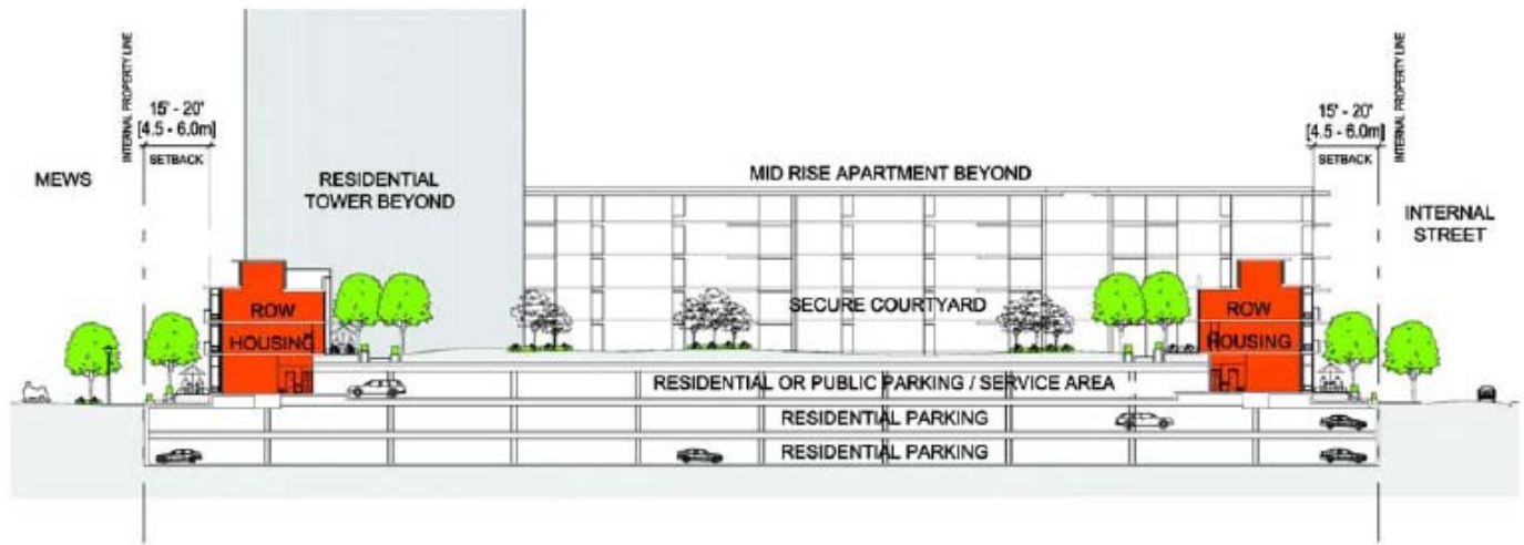
Figure 7 - Section of Parking Structure
