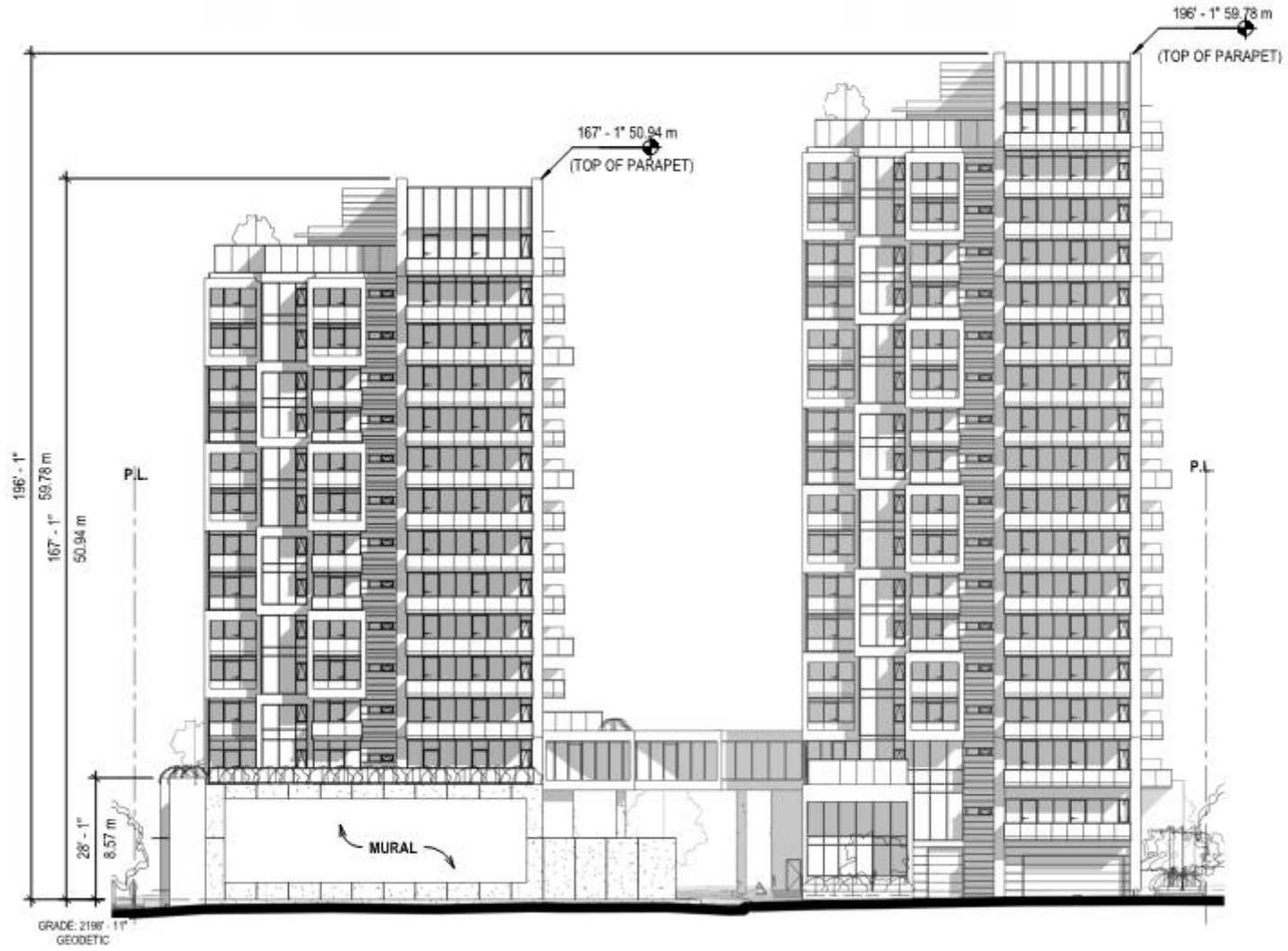
North Elevation
