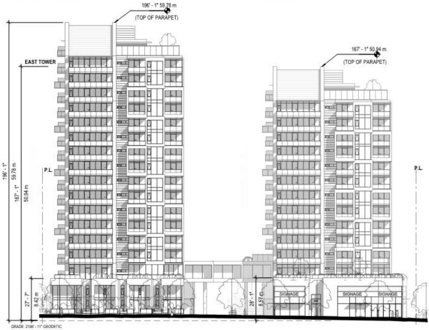
South Elevation
