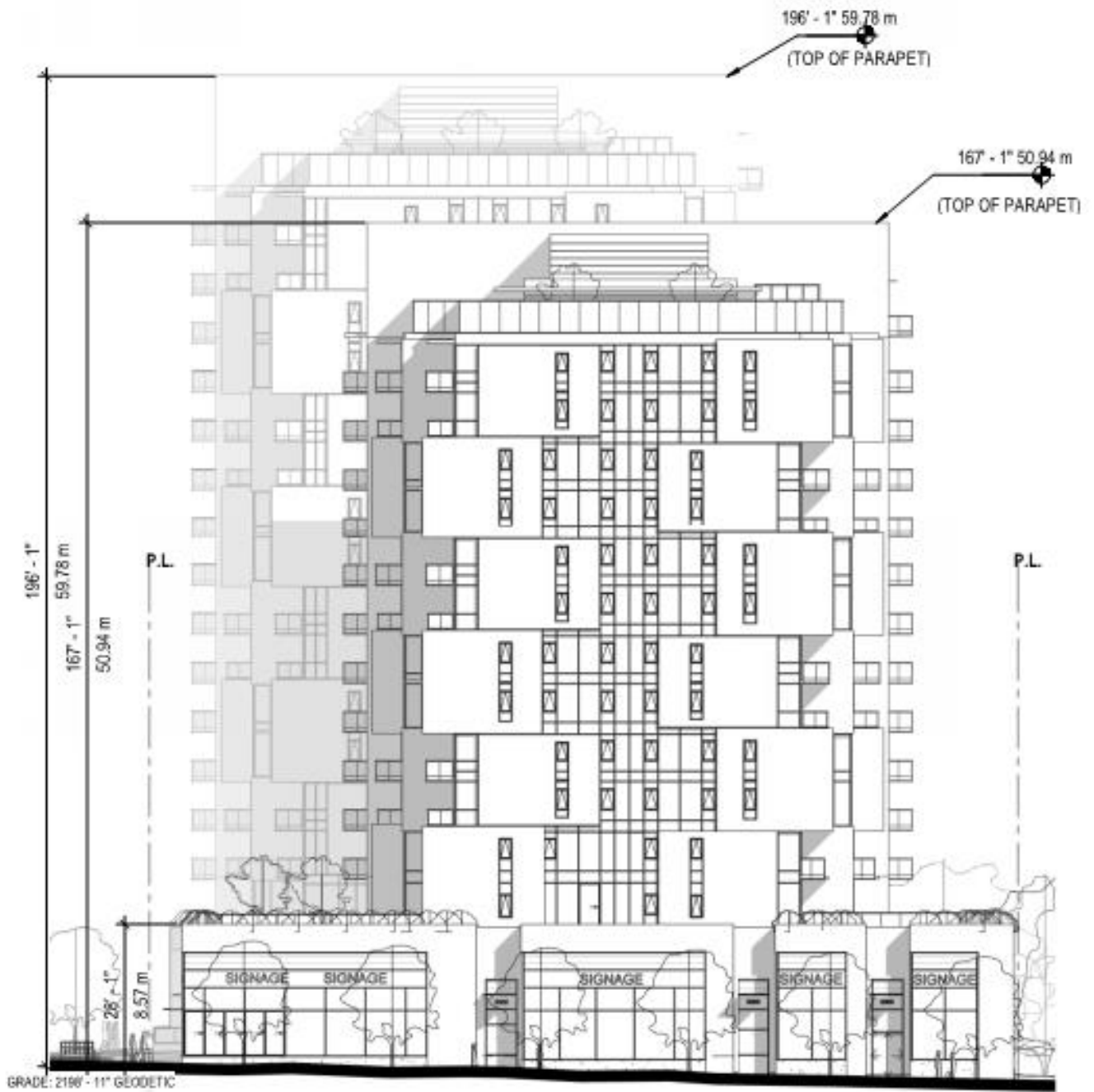
East Elevation
